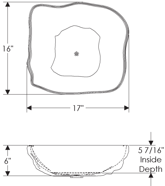
SK452 Small Pond Sink
